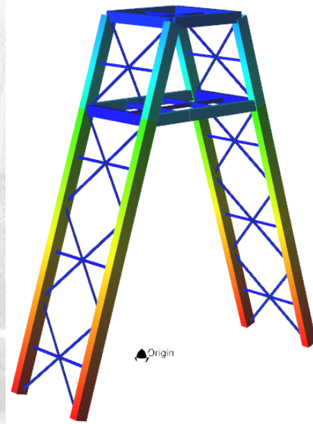
3D Finite Element model of Headframe structure
