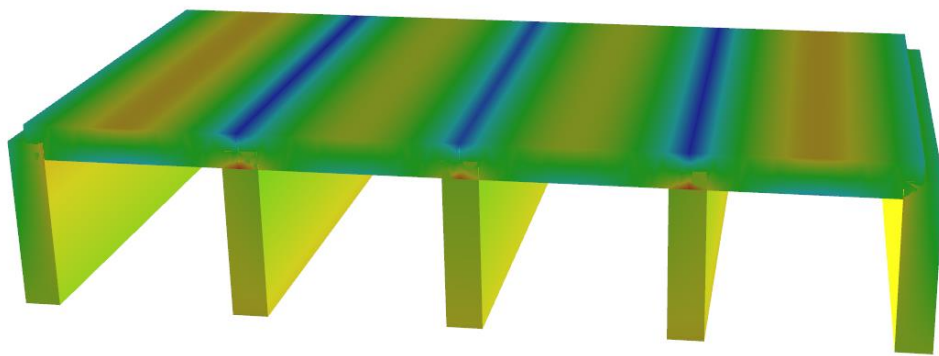
3D Finite Element model of Concrete Box Culvert
